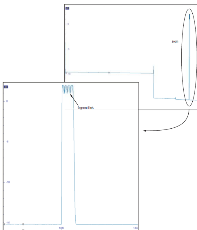
Figure 155: OTDR measurement of a 1x32 splitter with close segments
