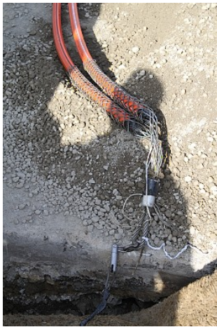
Figure 93: MD bundles attached to draw-rope
