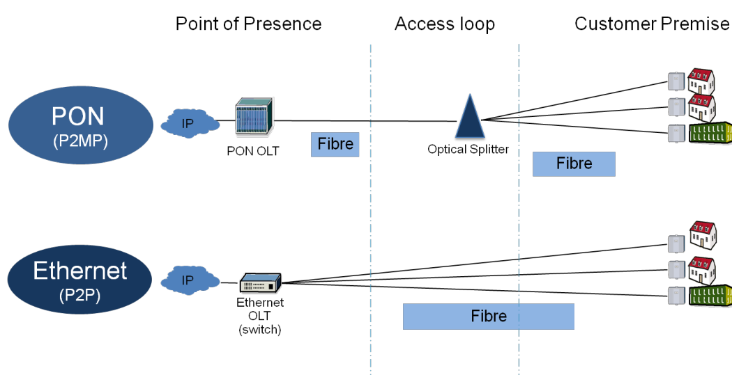
Figure 14: Different FTTH network architectures
