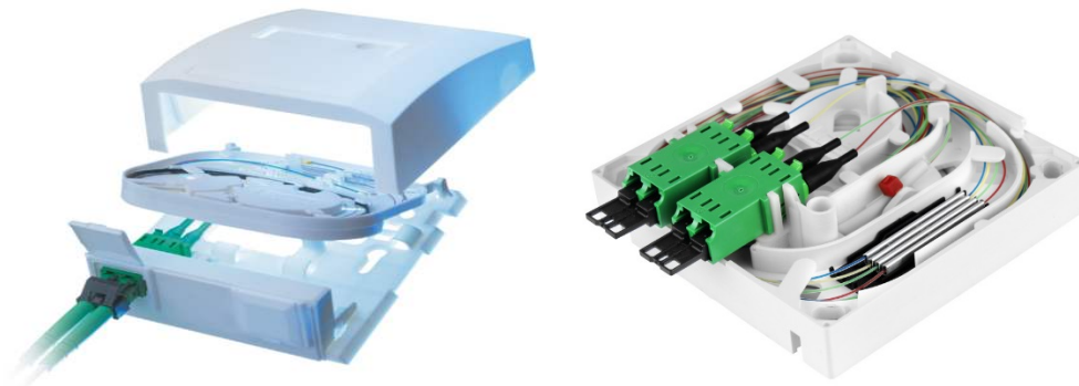
Figure 56: Detailed view of 2 different outlets: splice tray, bend radius guide, front plate with LC type
