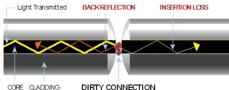
Figure 136: Increased insertion loss and back reflection due to dirty fibre connection.
