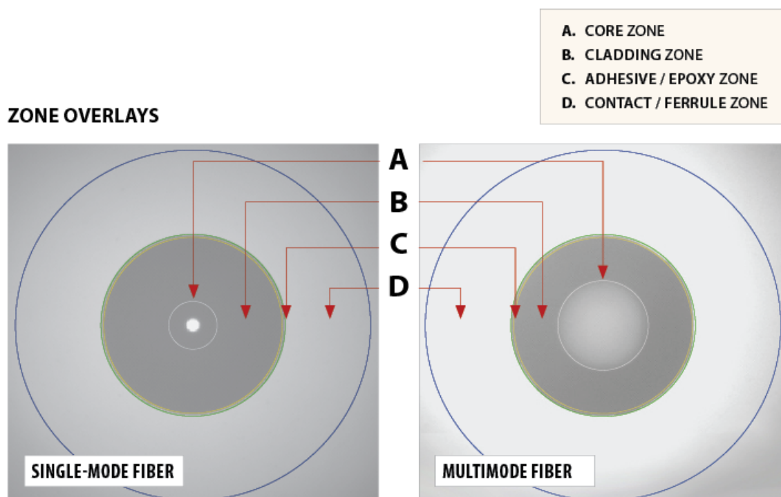
Figure 137: Connector end face inspection zones
