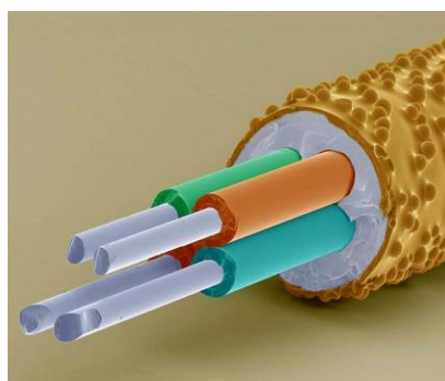
8.1.19 Figure 75: Fibre unit with 4 fibres
