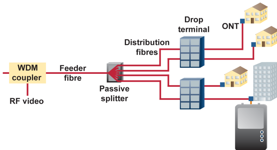
Figure 148: Activation testing using a PON power meter
