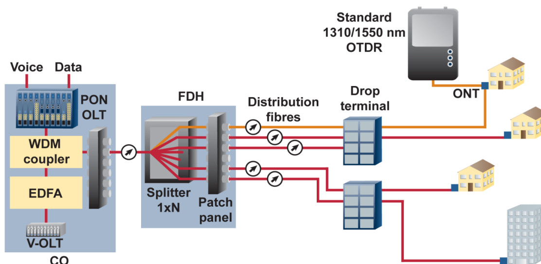
Figure 145: Measurement with an OTDR
