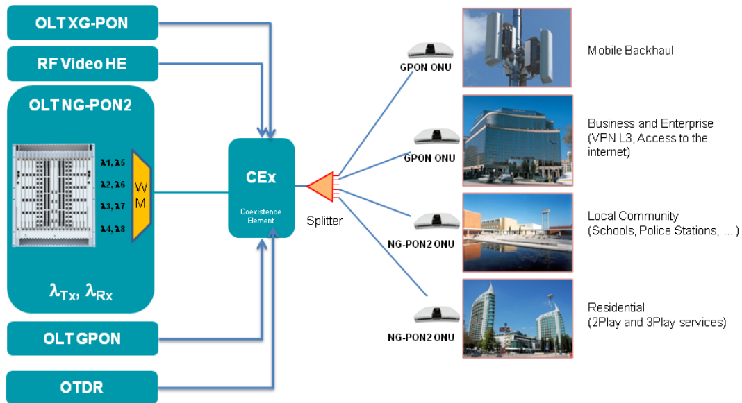
Figure 17: Coexistence of different FTTH technologies
