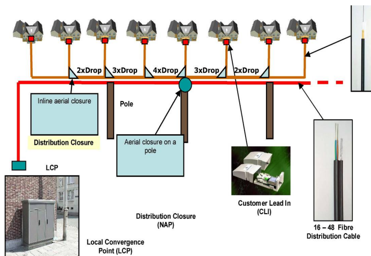
Figure 88: Product map for aerial cable
