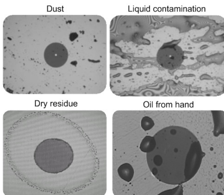
Figure 138: Appearance of various contaminants on a connector end face.
