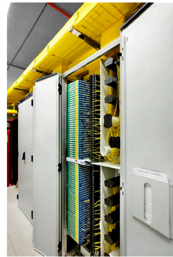
Figure 105: Example of ODF units
