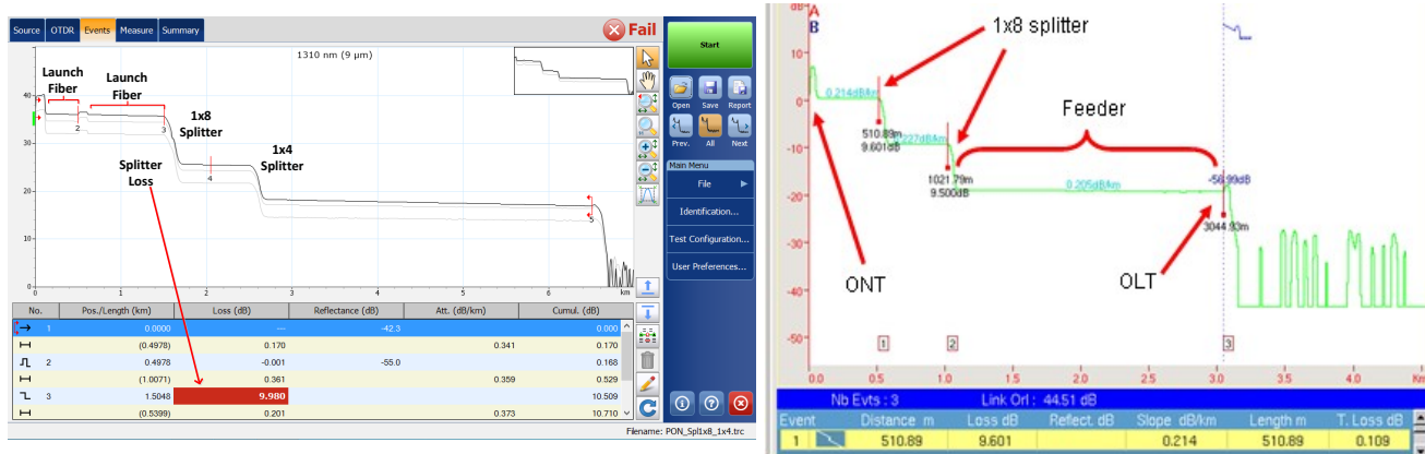
Figure 146: OTDR traces
