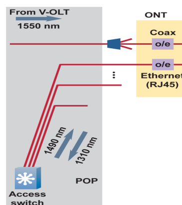
Figure 24: RF video overlay using a second fibre per subscriber, deployed in a tree structure.
