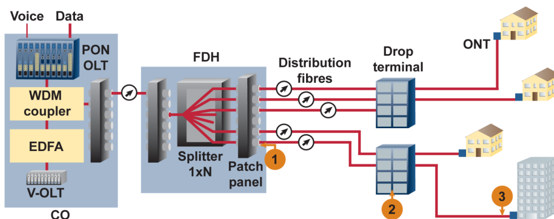
Figure 149: Testing point in PON
