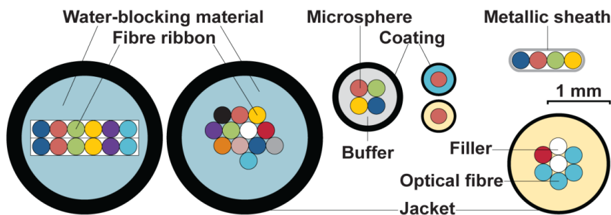
Figure 78: Examples of Fibre units. Micro-duct spelling in diagram
