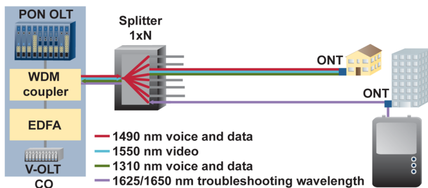
Figure 160: PON network troubleshooting
