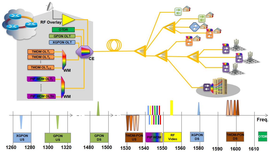
Figure 16: ITU-T G.987 wavelength plan
