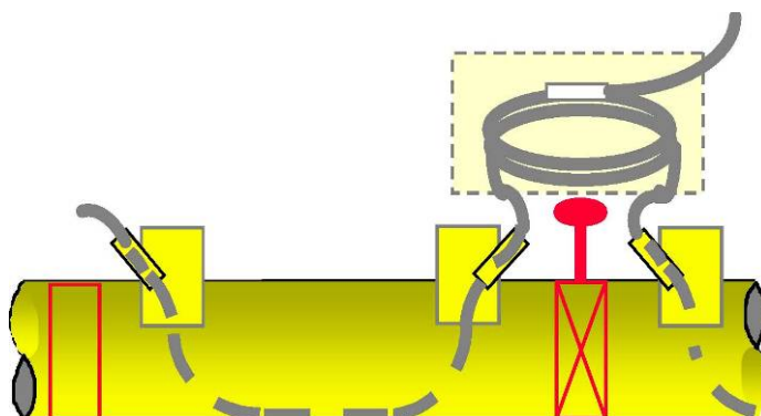
Figure 85: Gas pipeline section, including I/O ports and the bypassing of a valve defining one point-of-presence for the fibre-optic cable
