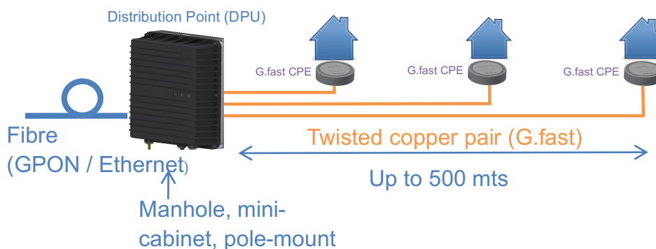
Figure 19: FTTH Applications
