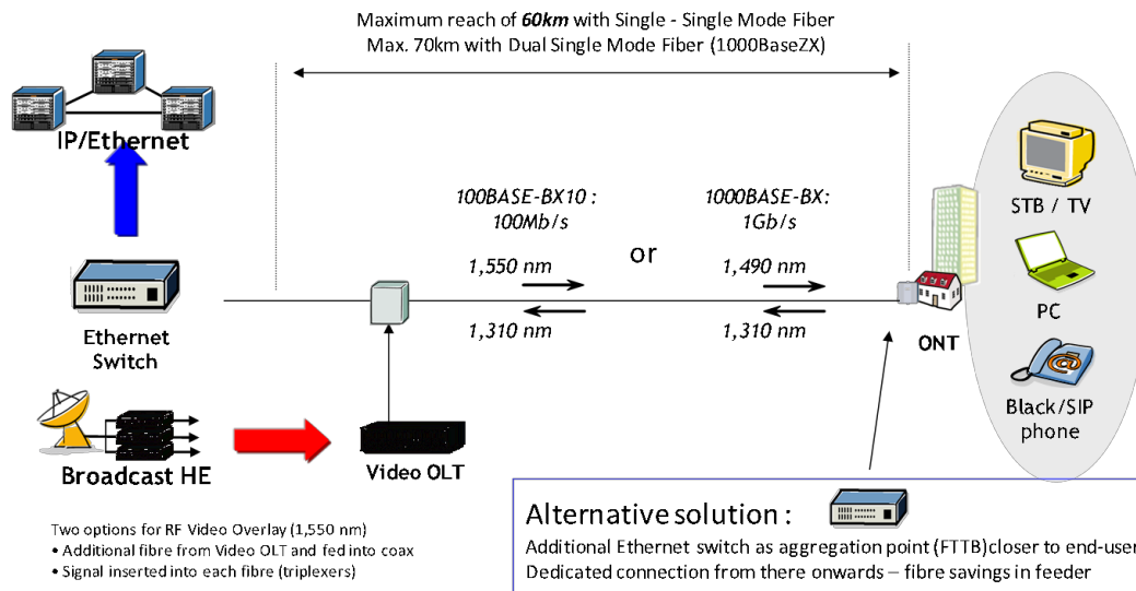
Figure 23: Ethernet network diagram
