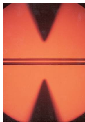
Figure 131: Splice complete
