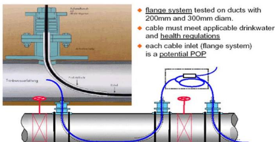
Figure 86: Cross-section showing fibre installed in a drinking water system
