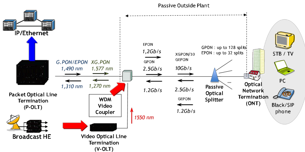
Figure 15: Schematic diagram of a GPON network
