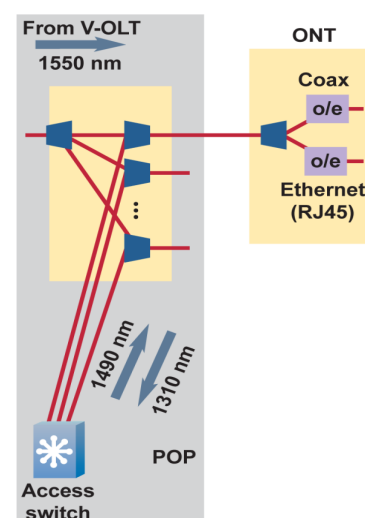
Figure 25: Insertion of RF video signal into point-to-point fibres.
