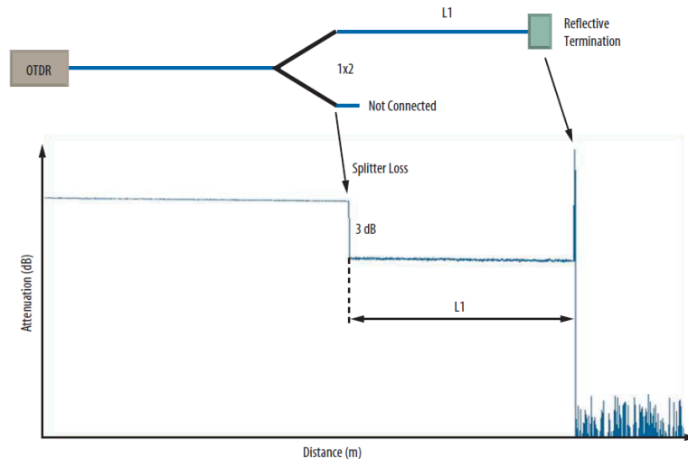
Figure 152: OTDR trace with a 1x2 splitter with only one connected segment
