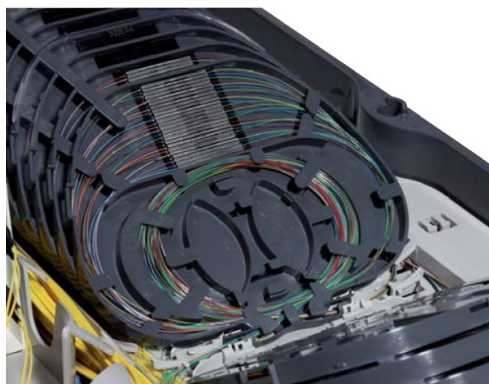
Figure 52: Example of stacked splice trays with individual fibre management
