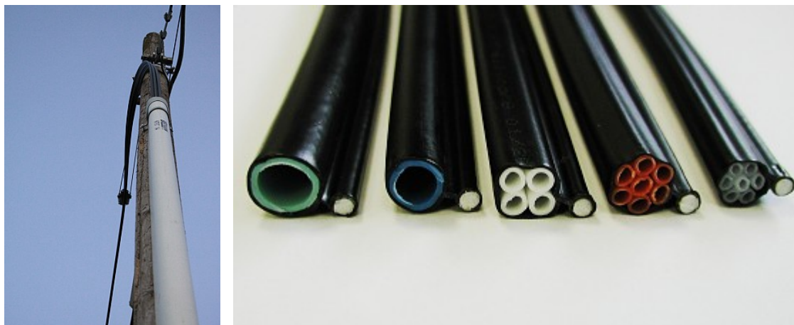
Figure 97: Aerial micro-ducts
