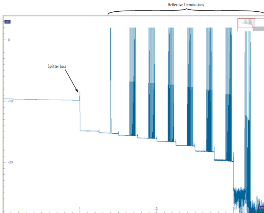
Figure 156: OTDR trace on PON equipped with reflective filters
