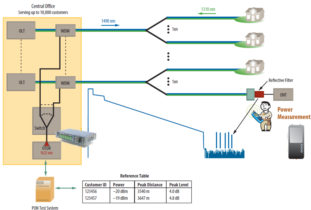
Figure 158: PON Test System used for Provisioning
