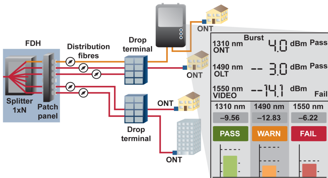
Figure 150: Pass-through testing of all wavelengths
