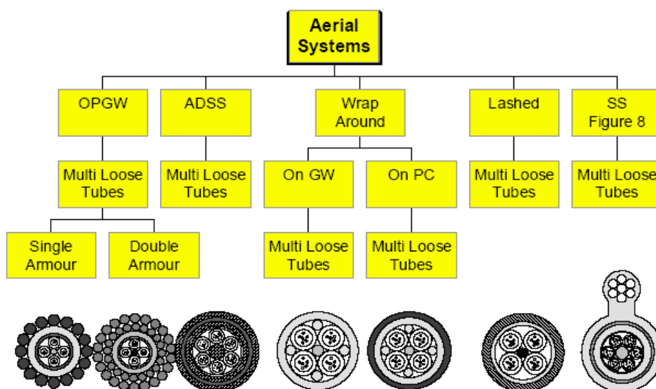
Figure 90: Aerial cable selection
