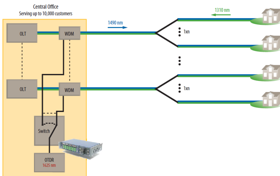
Figure 157: PON Test System integrating a switch
