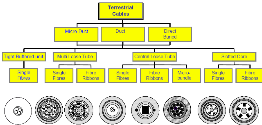
Figure 73: FOC cable selection
