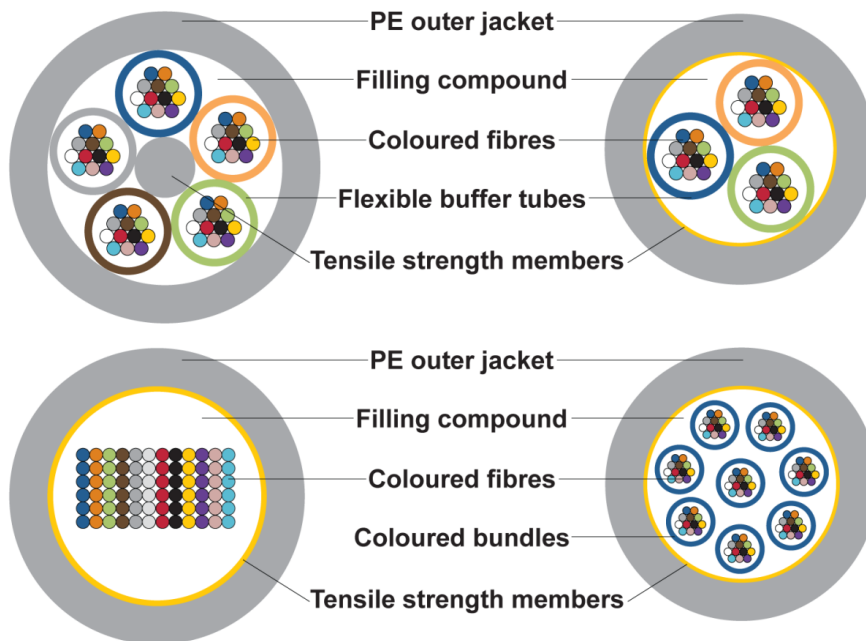
Figure 77: Optical fibre micro-cables (not to scale)
