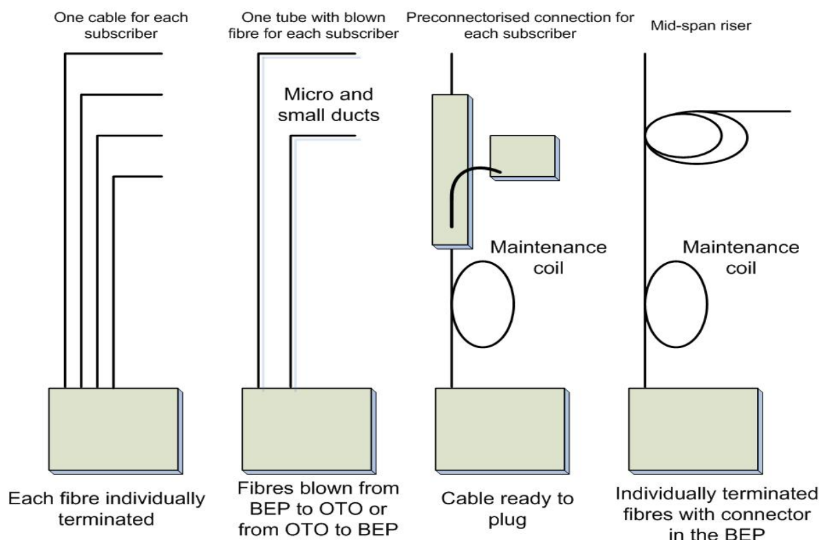
Figure 41: Example of riser architecture
