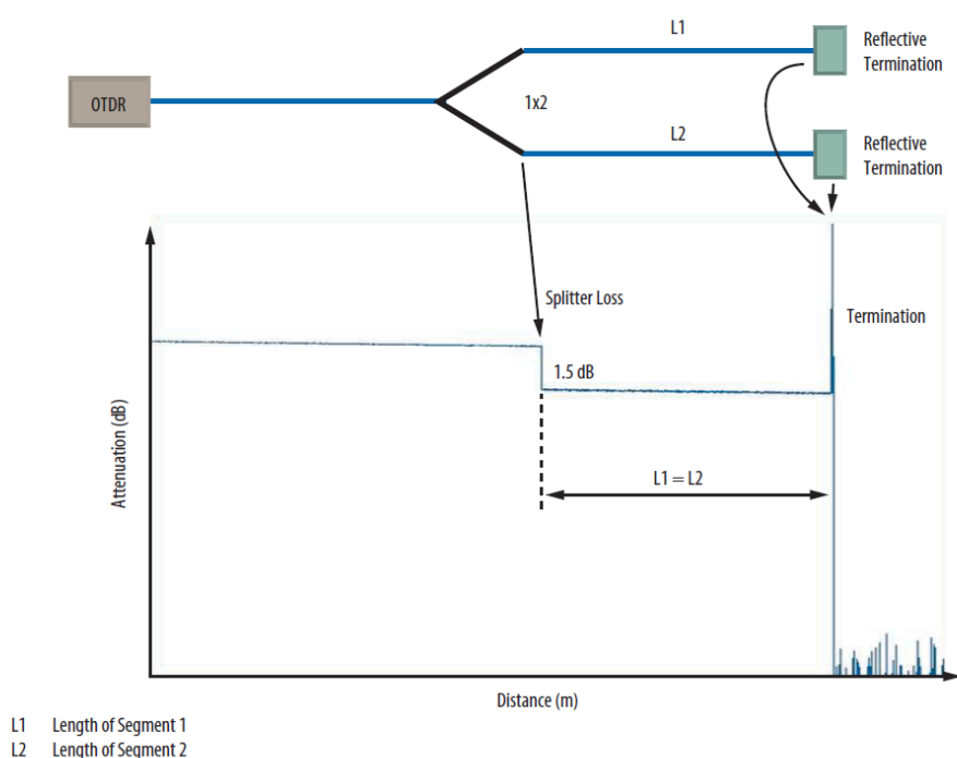
Figure 154: OTDR trace with a 1x2 splitter with 2 segments of equal lengths
