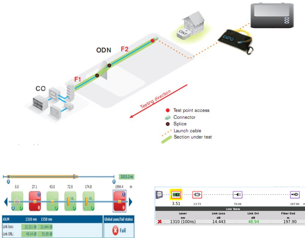
Figure 147: Icon based OTDRs
