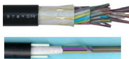
Figure 34: Modular cable in duct system
