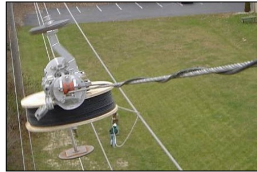
Figure 89: Wrapped aerial cable
