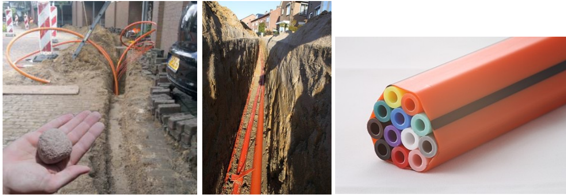
Figure 96: Ducts laid in open trenches
