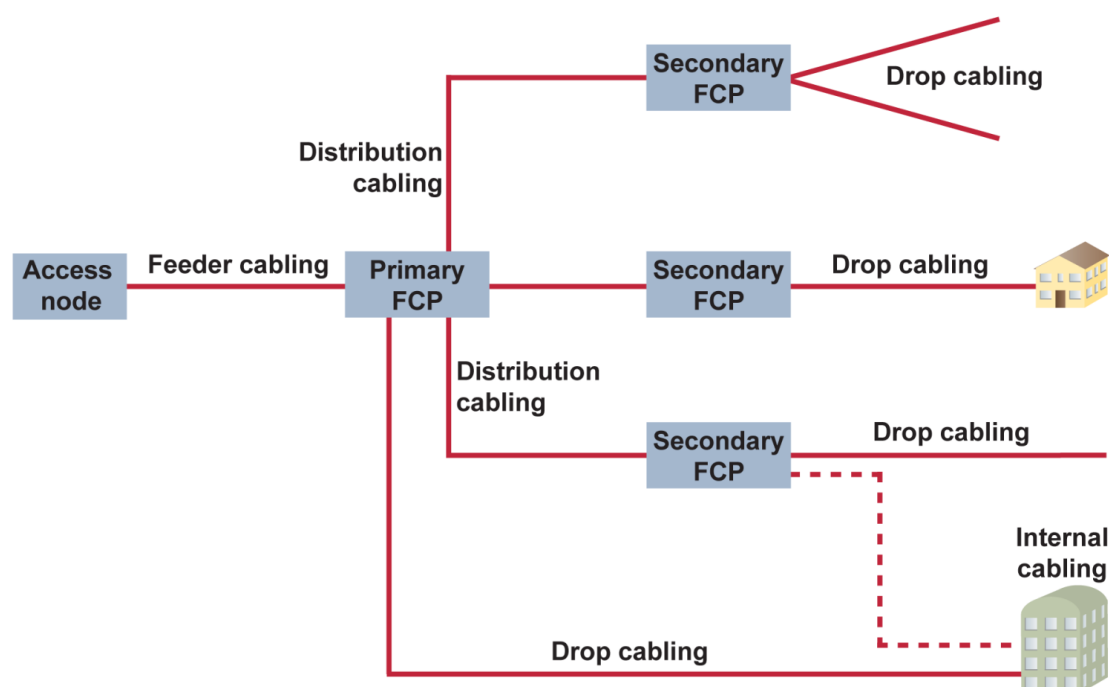
Figure 28: Main elements in a FTTH network infrastructure.
