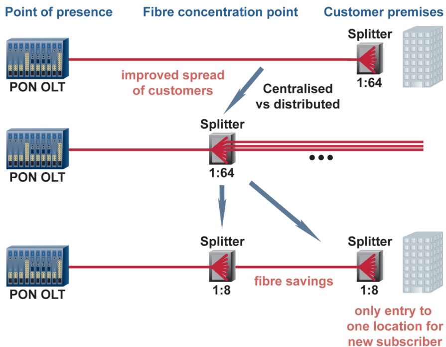
Figure 22: Centralized and distributed splitting in a PON
