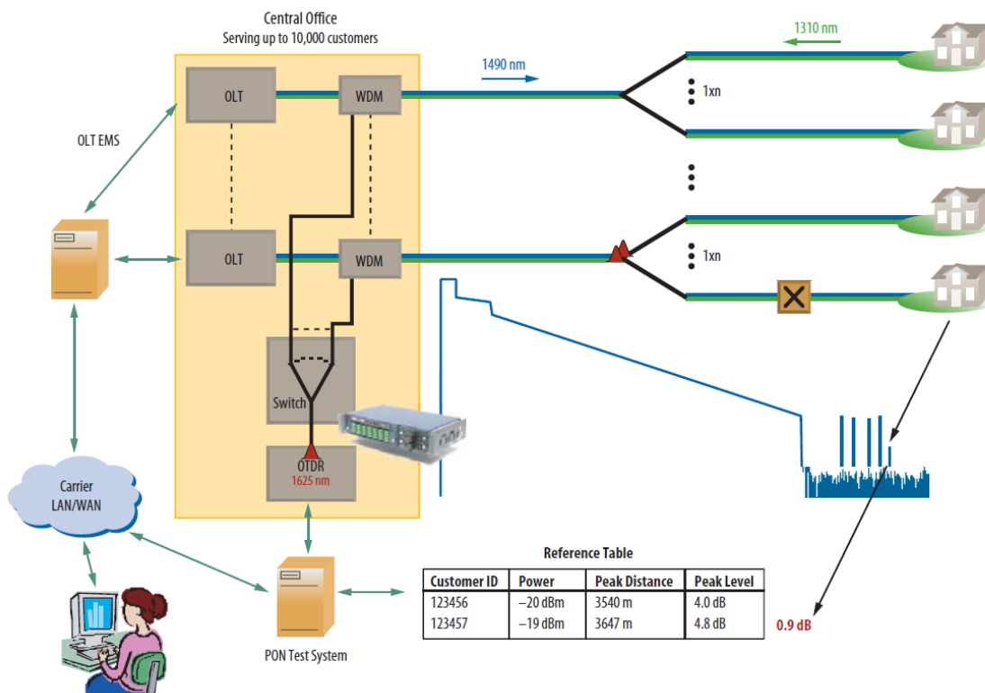
Figure 159: PON Test System used for troubleshooting
