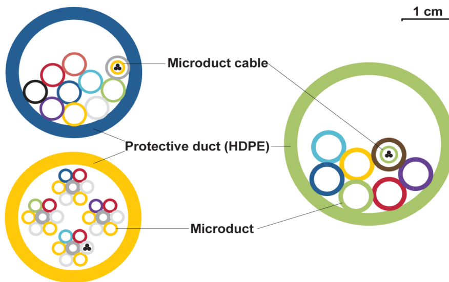
Figure 76: Protected micro-ducts with loose package
