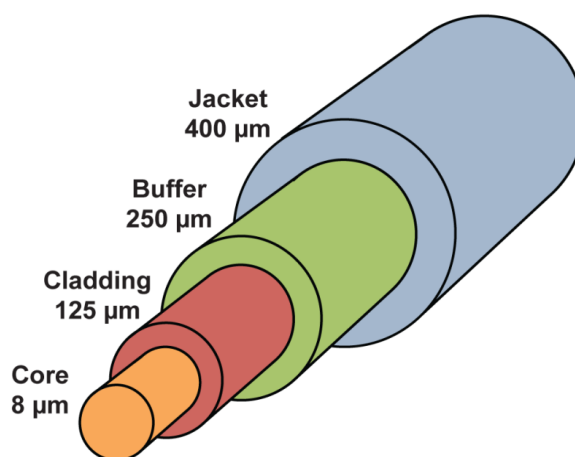
9.1.2 Figure 100: Single-mode optical fibre construction
