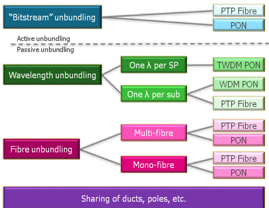
Figure 27: Classification of infrastructure sharing for PTP Fibre and PON FTTH.
