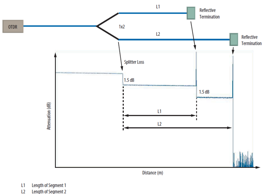
Figure 153: OTDR trace with a 1x2 splitter with the 2 segments of different lengths
