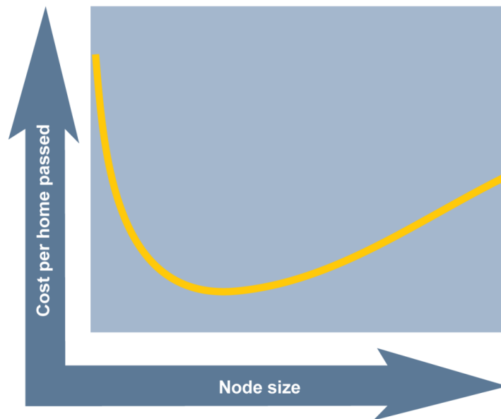
Figure 21: Optimisation of node side in a PON with single-level splitting
