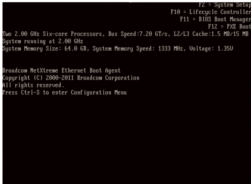
Figure 5.6: POST screen
