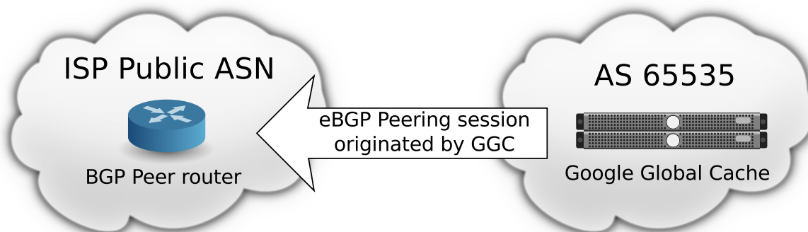
Figure 6.1: BGP overview
